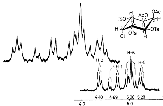
Fig. 2. Partial PMR spectrum of 1,2-di- O -acetyl-5-chloro-5-deoxy-3,4,6-tri- O - p -tolylsulfonyl- neo -inositol ( 20b ) in \text{CDCl}_3 at 60 MHz. An amplified (magnification, 2) spectrum is shown above.
